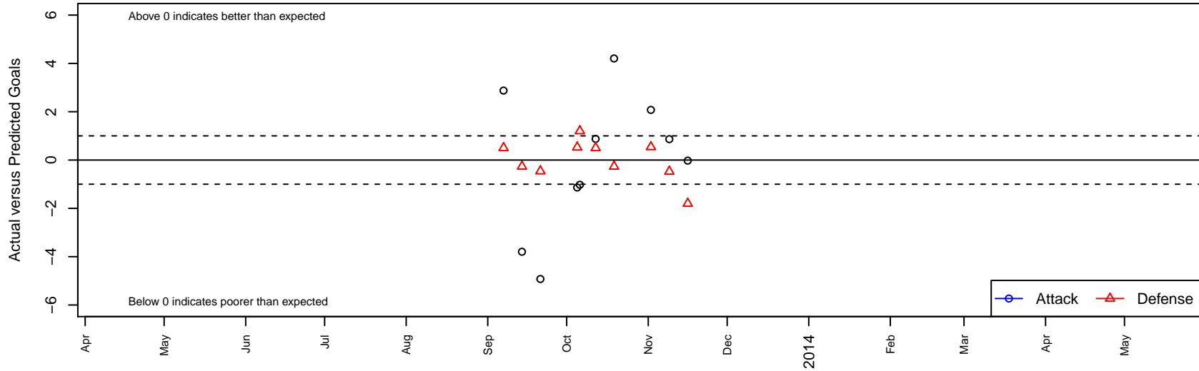
East Valley FC Earthquakes B00 Dots are actual minus expected GF (blue circles) and GA (red triangles). Blue line is smoothed change in attack strength. Red is smoothed change in defense strength.
